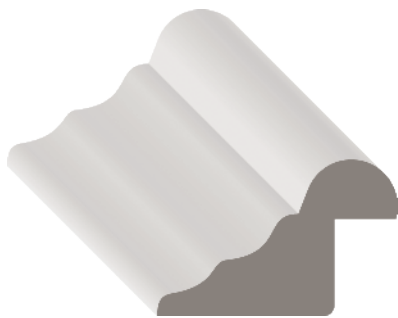
Stock Code MP3724 (1626516) Dimensions 3/4" x 1 3/16" x 16' PFJ
