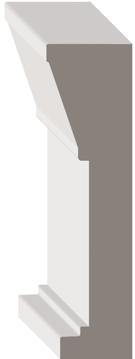
Stock Code MFPU5015 (1328514) Dimensions 1 \frac{1}{2} " x 5 \frac{1}{2} " x 12' MDF/UL
