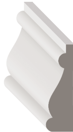
Stock Code MP3005 (1328764) Dimensions ½" x 1½" x 14' PFJ
