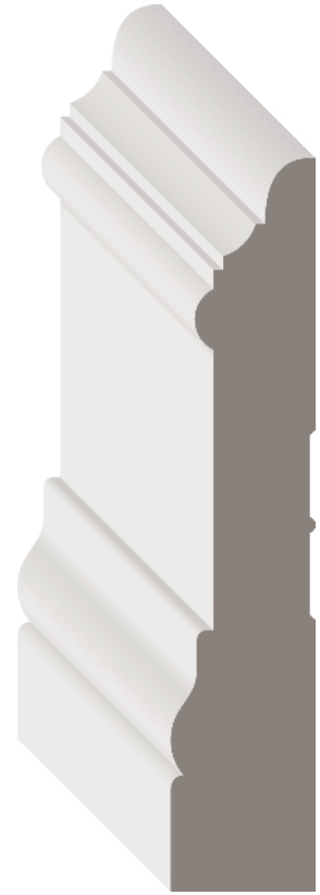
Stock Code MFPU535 (1626198) Dimensions 1 1/16" x 3 1/2" x 15' MDF/UL
